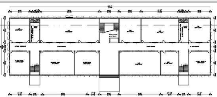
SECOND FLOOR PLAN BLOCK - A
