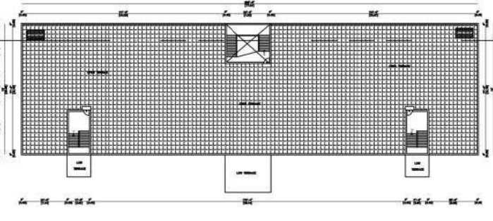
TERRACE FLOOR PLAN BLOCK - A
